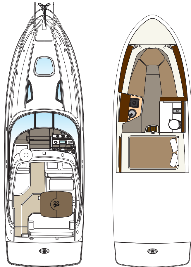
COCKPIT LAYOUT
